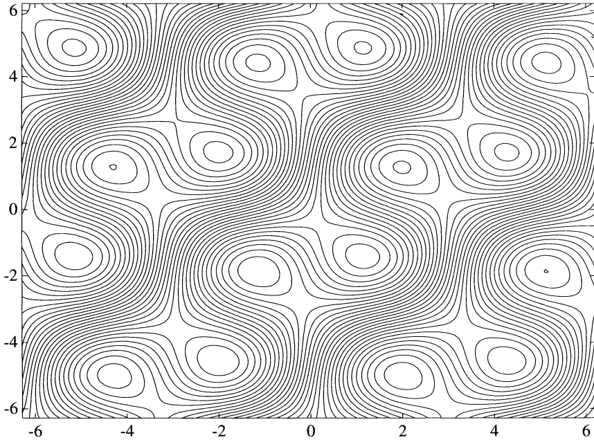
FIG. 8.2. Cellular flow with drift \mathbf{c} = 0.2(1, 2) .
