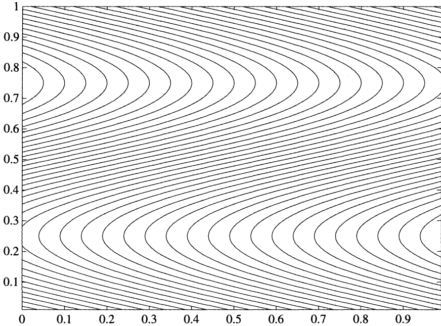
FIG. 8.4. Shear layer flow with drift \mathbf{c} = (0, 0.3) .
