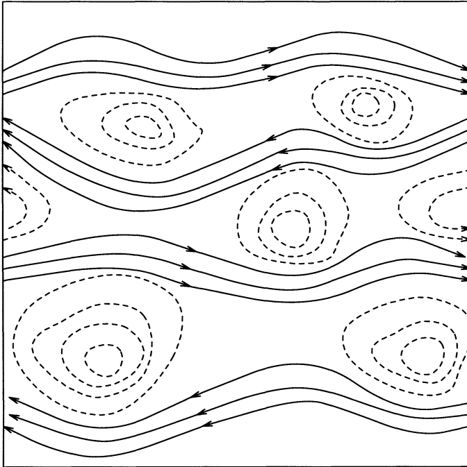
FIG. 7.1. Multichannel flow.
