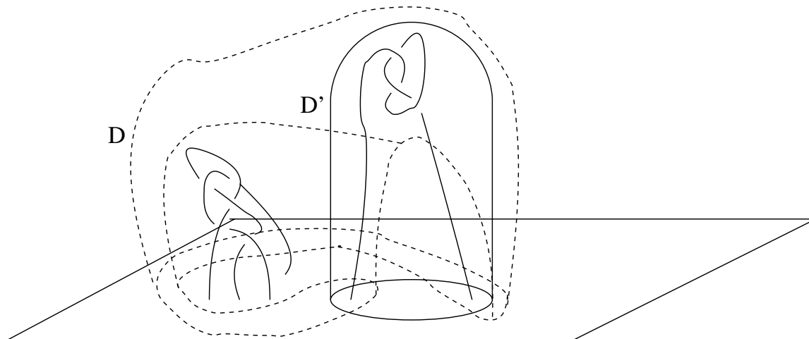
Figure 16: Two disks of the same height
