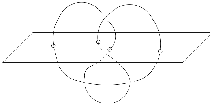
Figure 14: The Figure 8 knot in bridge position
