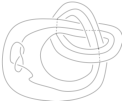
Figure 11: A swallow-follow torus
