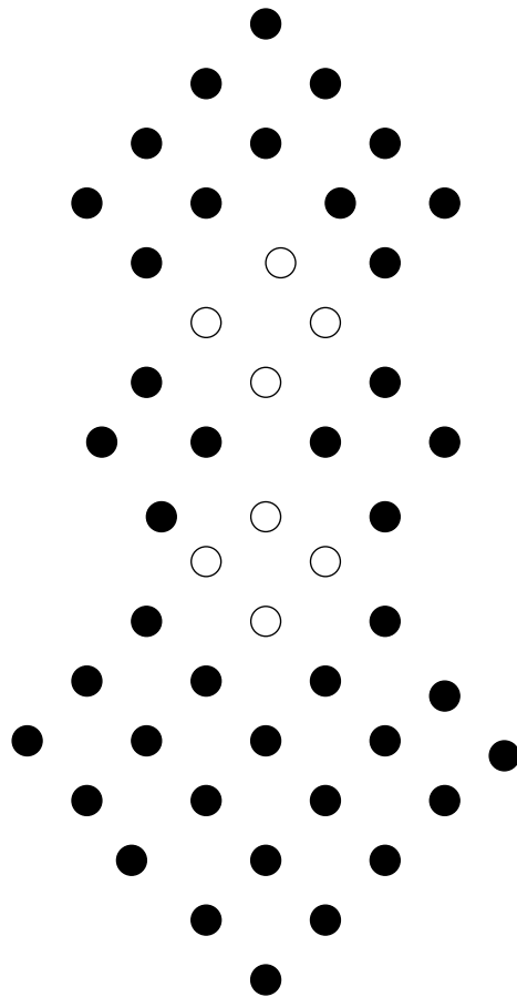
Figure 5: A cancellation principle
