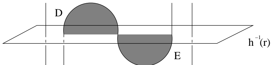
Figure 8: Two disks describing an isotopy
