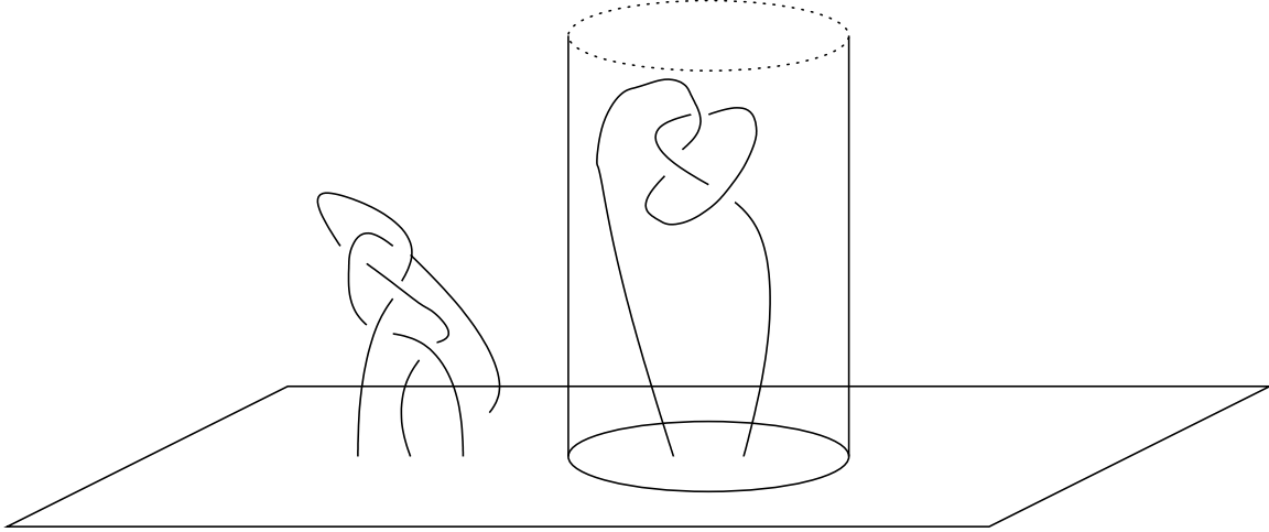
Figure 15: The portions \alpha and \beta of L
