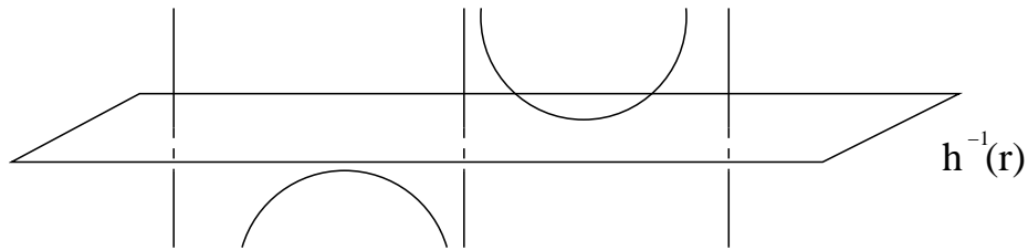
Figure 7: After the isotopy
