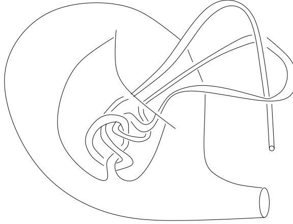
Figure 12: Convoluted portion of a swallow follow torus
