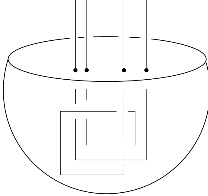
Figure 13: A bowl like 2-sphere (flat face up)
