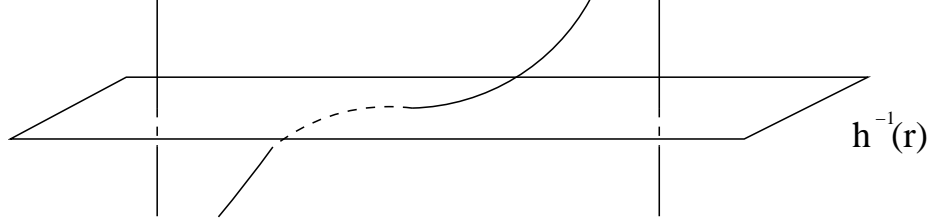
Figure 9: After the isotopy
