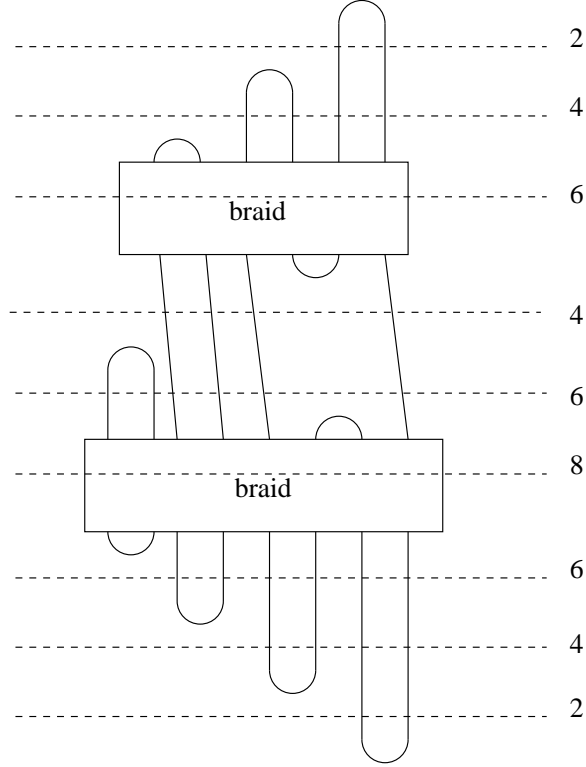
Figure 1: Thin position for knots
