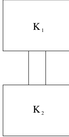
Figure 10: Connected sum of knots
