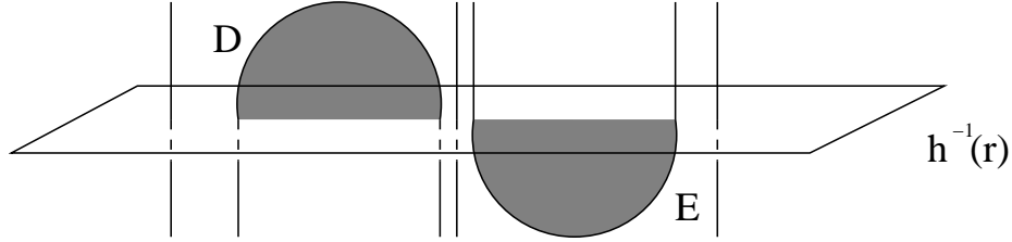
Figure 6: Two disks describing an isotopy
