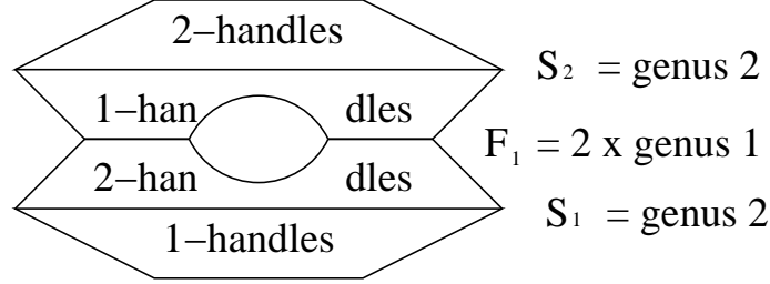
Figure 2: Thin position for 3-manifolds
