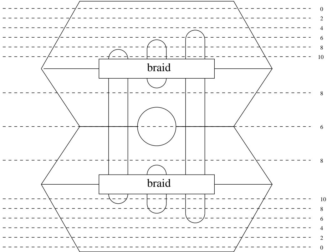
Figure 3: Thin position for knots in 3-manifolds
