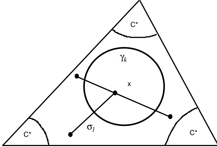
Figure 1: Corners of the triangle \Sigma .
