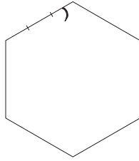
FIGURE 3.1. A ciliation in a face. The cilium is placed on a bordering edge, 0.5 unit length away from the nearest vertex.
