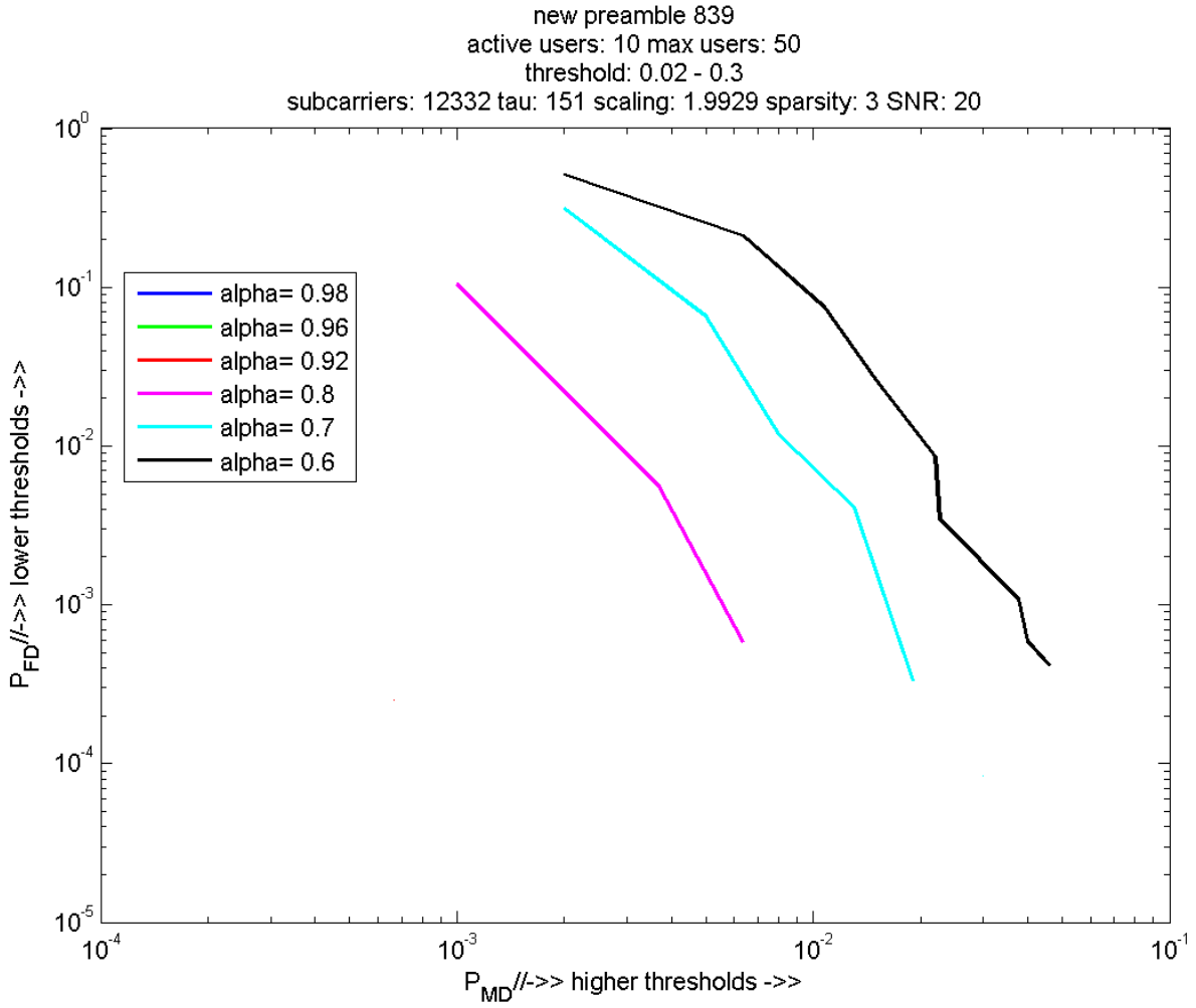
Fig. 3. P_{FD} = 10^{-2} over P_{MD} = 10^{-2} for the 5G "one-shot" random access with same parameters
