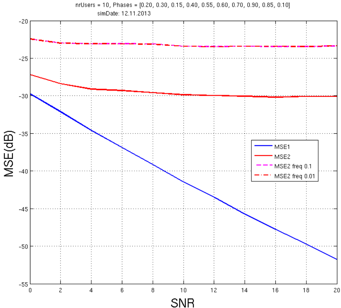
Fig. 5. MSE performance of the relay and compress scheme under "perturbations" for 1) Bob having ideal measurements and 2) Eve having perturbed measurements with a) phase errors and, worse, b) rank-one distortion
