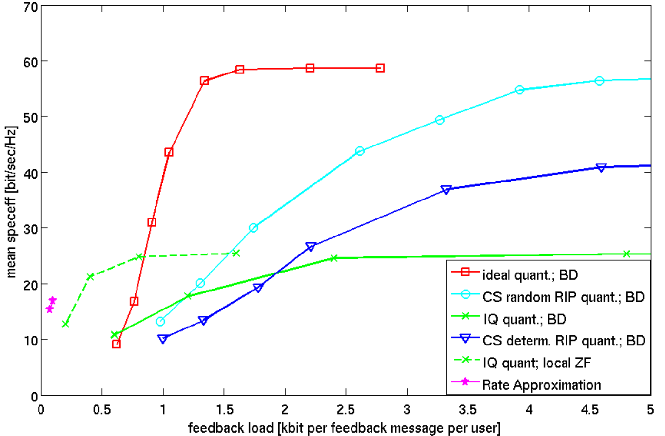
Fig. 4. Mean spectral efficiency of CoMP schemes over feedback load using IQ quantization or CS based techniques: BD is block diagonalization, ZF is zero forcing and Rate Approximation is the scheme from [33]
