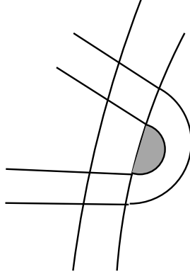
Figure 4: An innermost bigon
