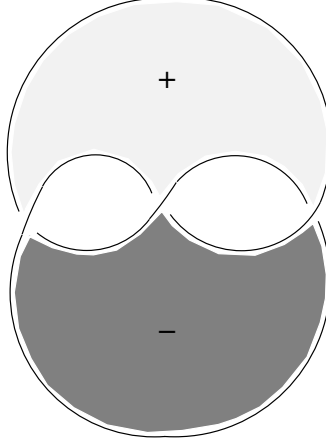
Figure 1: A Seifert surface for the trefoil
