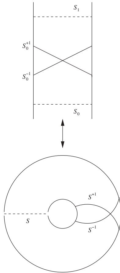
FIGURE 2. M(K) and E(K) .
