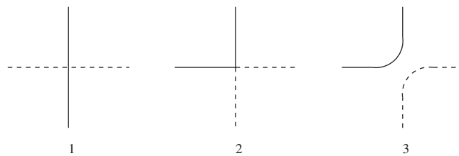
FIGURE 1. (1) Cross-section of surfaces before exchange. (2) Cross-section of surfaces after exchange. (3) Cross-section of surfaces after round-off.
