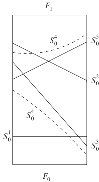
FIGURE 7. Five separating surfaces.
