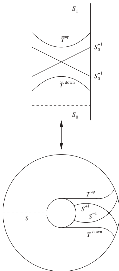
FIGURE 3. \tilde{T}^{\text{down}} and \tilde{T}^{\text{up}} .
