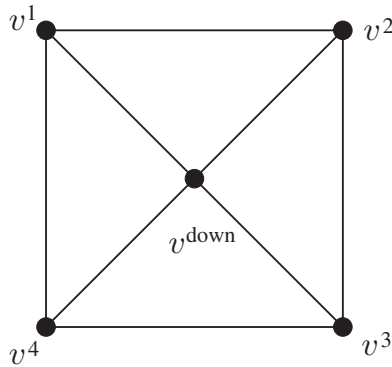
FIGURE 5. A homotopically trivial loop.
