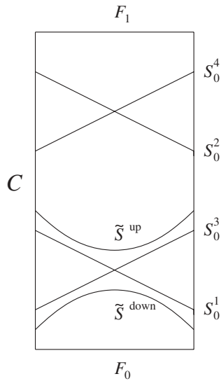
FIGURE 6. The product region.
