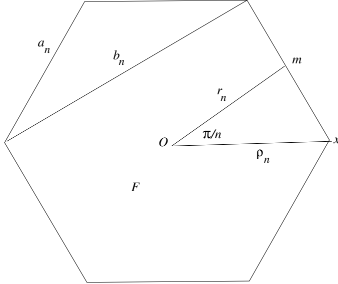
Figure 1: Geometry of a hyperbolic n -gon.
