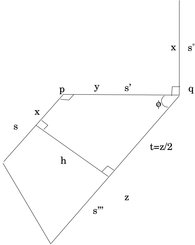
Figure 3: Three orthogonal segments.
