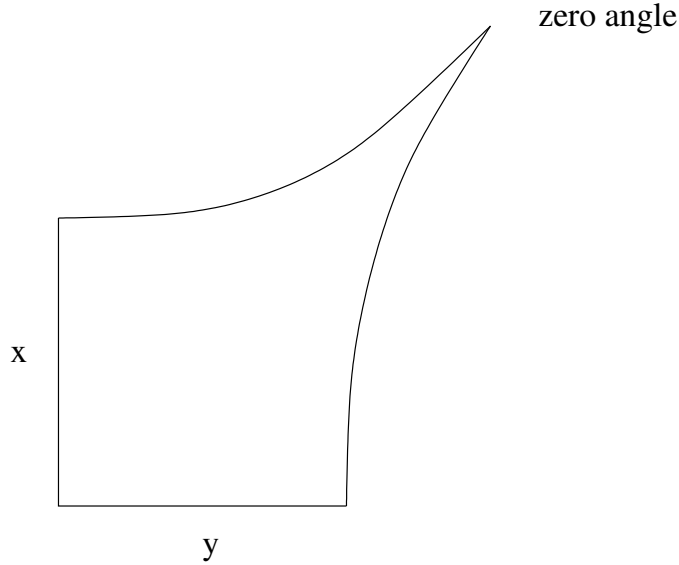
Figure 2: A Lambert quadrilateral.
