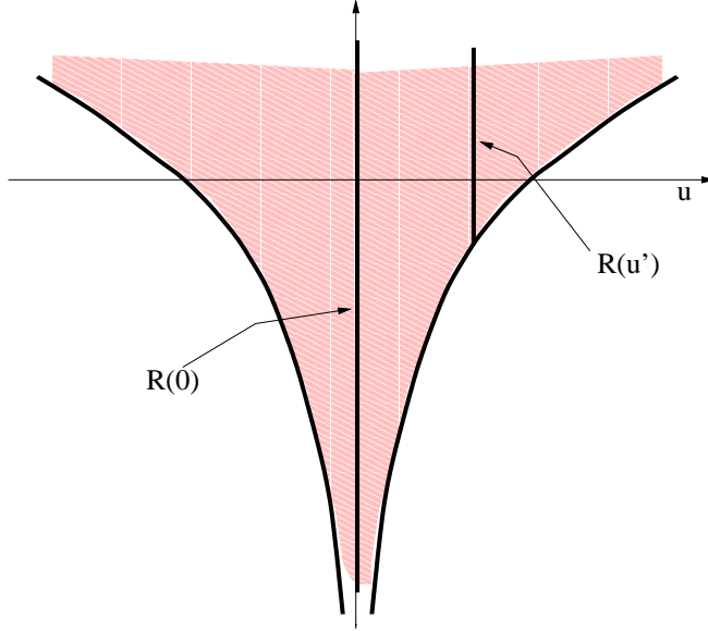
Figure 2: A locally sub-Lipschitz mapping continuous
