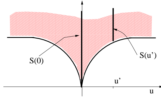
Figure 1: A mapping that isn't locally sub-Lipschitz continuous
