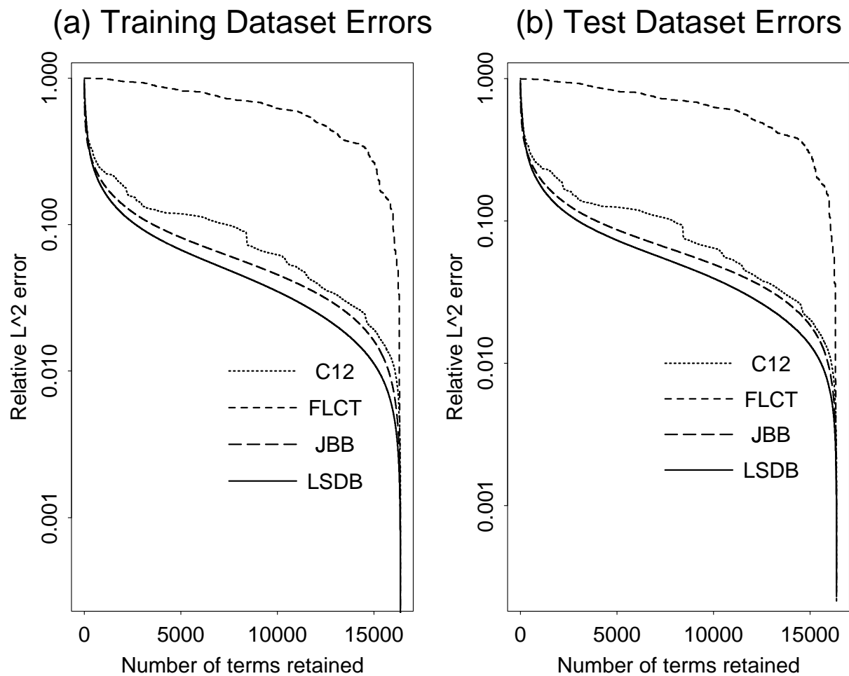
Figure 10: Relative \ell^2 approximation errors of the “Rogues’ Gallery” dataset using various bases versus the number of terms used for approximation. (a) Average over all the training images; (b) Average over all the test images.
