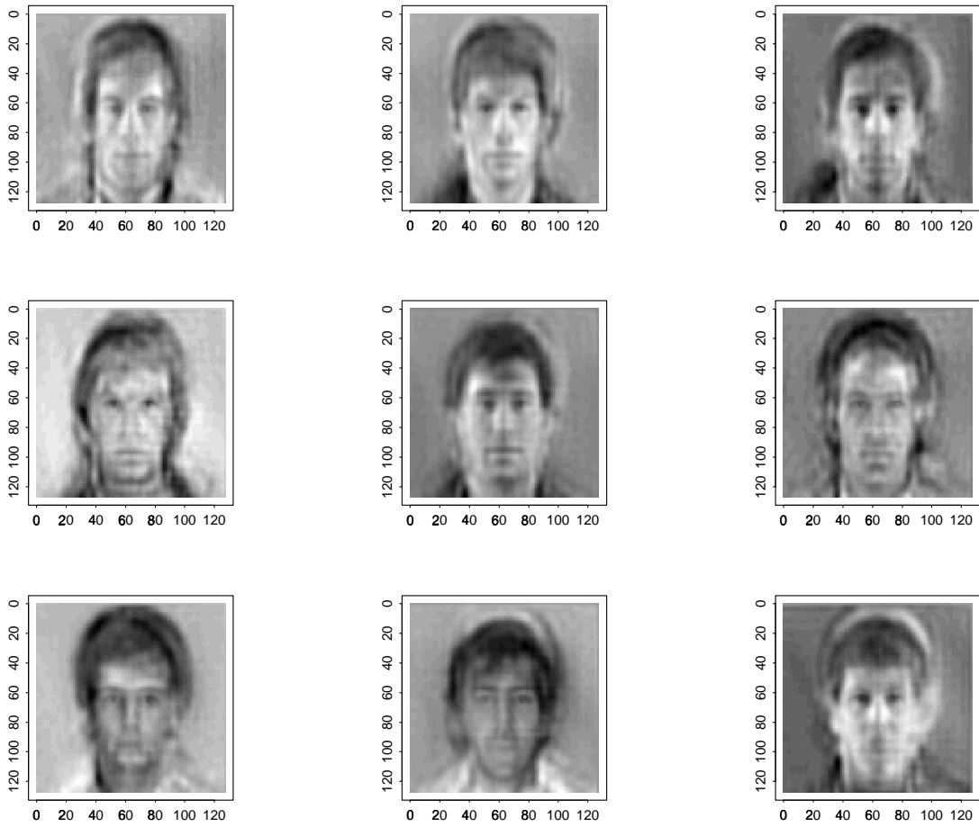
Figure 15: Nine sampled faces from the KLB-JBB800 model. Compare with Figure 14.
