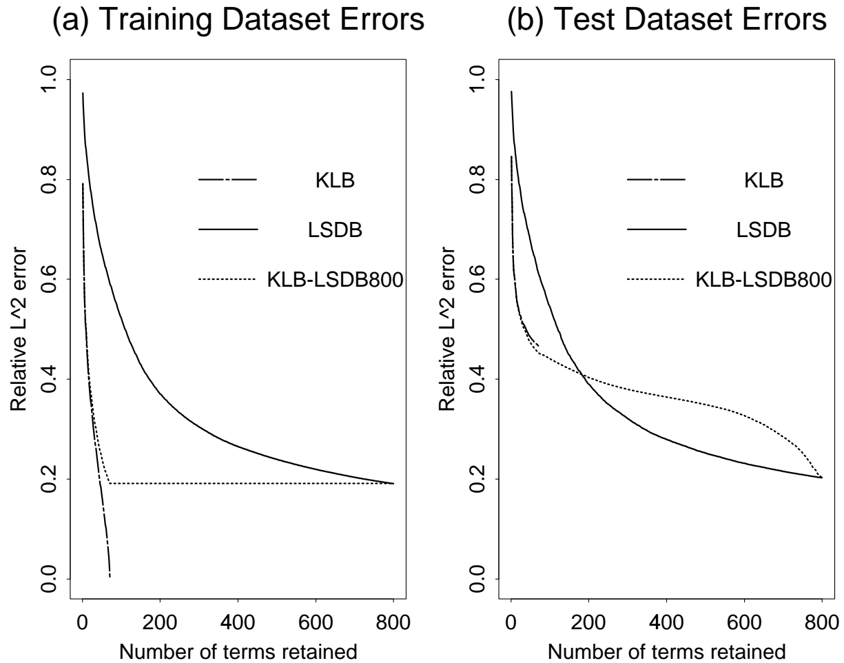
Figure 11: Relative \ell^2 approximation errors versus the number of terms used for approximation for the first 800 terms. (a) Average over all the training images; (b) Average over all the test images. Now we compare the performance of the KLB (only 72 terms available), LSDB, and the KLB computed on top of the 800 LSDB coordinates.
