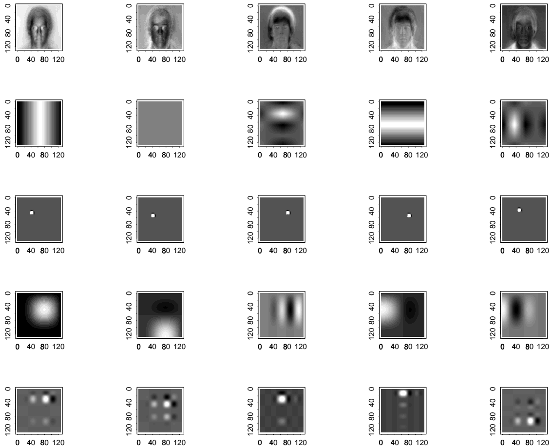
Figure 8: Comparison of the five most energetic basis vectors in the five bases. First row: KLB, second row: C12 wavelet basis, third row: FLCT 8 \times 8 , fourth row: JBB, and the last row: LSDB.
