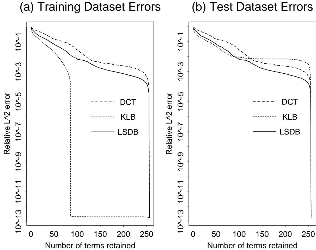
Figure 4: Relative \ell^2 approximation errors of the geophysical acoustic waveforms using DCT, KLB, LSDB plotted as functions of the number of terms used for approximation. (a) Average errors over all the training signals; (b) Average errors over all the test signals.
