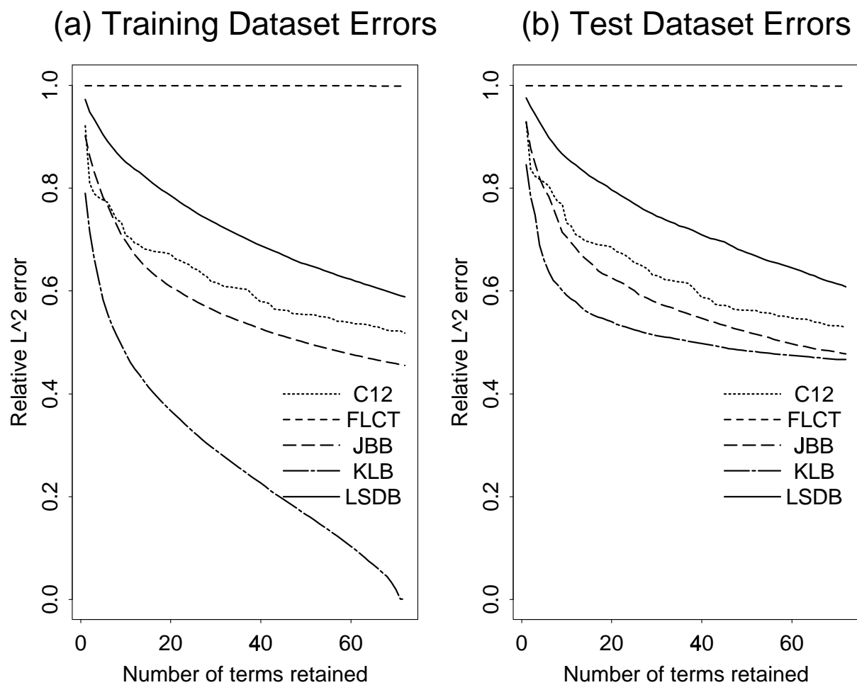
Figure 9: Relative \ell^2 approximation errors of the “Rogues’ Gallery” dataset using various bases versus the number of terms used for approximation for the first 72 terms. (a) Average errors over all the training images; (b) Average errors over all the test images.
