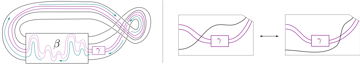
FIGURE 14. Left: a Legendrian \vartheta -loop for the Legendrian link \Lambda(\beta, i; \gamma) \subset (\mathbb{R}^3, \xi_{\text{st}}) , where the purple \gamma -box moves around clockwise around the \beta -box and comes back to itself using the upper strands). Right: the local move, consisting of a sequence of l(\gamma) Reidemeister III moves, which we use in order to push the purple \gamma -box, right to left, through the \beta -box.
