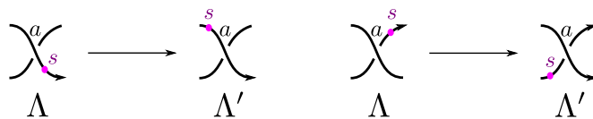
FIGURE 18. A base point move.
