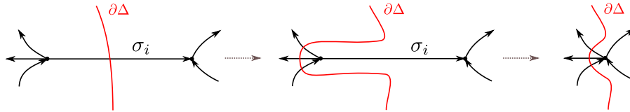
FIGURE 17. Sliding the arc \partial\Delta to avoid intersections with \sigma_i , and then contracting \sigma_i .
