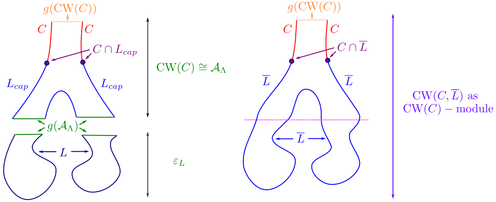
FIGURE 36. On the left, the holomorphic disks contributing to the augmentation \varepsilon_L (bottom) and the surgery isomorphism \text{CW}(C) \cong \mathcal{A}_\Lambda (top). On the right, the holomorphic disks contributing to the module structure \text{CW}(C) \rightarrow \text{End}(\text{CW}(C, \bar{L})) . The notation g(\text{CW}(C)) and g(\mathcal{A}_\Lambda) stands for generators of the algebras \text{CW}(C) and \mathcal{A}_\Lambda : g(\text{CW}(C)) are Reeb chords of \partial C or the minimum of C , and g(\mathcal{A}_\Lambda) are Reeb chords of \Lambda .
