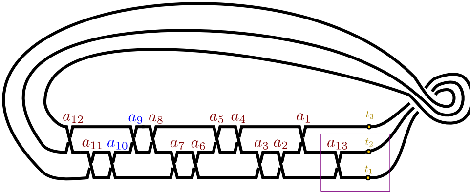
FIGURE 30. Lagrangian projection for the Legendrian link \Lambda_1 , as used in the proof of Theorem 6.4. In this proof, the crossings a_{10}, a_9 , in blue, are used to detect the infinite order of the \vartheta -monodromy. The \vartheta -monodromy is obtained by moving the purple box around this projection. To construct \Lambda_2 instead, add an additional crossing labeled a_{14} to the purple box, between a_{13} and the base points t_1, t_2 .
