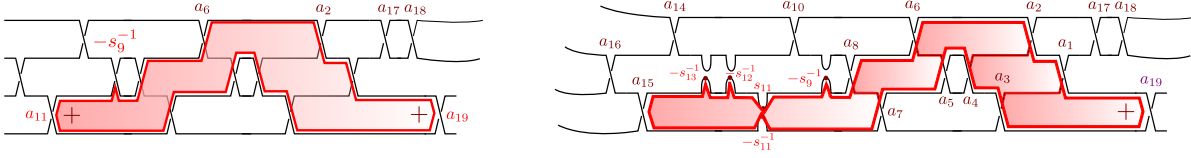
FIGURE 29. Disks with positive corners at a_{11}, a_{19} (left) and a_{15}, a_{19} (right), contributing to \Phi_{11}(a_{19}) and \Phi_{15}(a_{19}) respectively. For these disks, the positive corner at a_{19} has positive orientation sign, while the positive corner at a_{11} and a_{15} has negative orientation sign.
