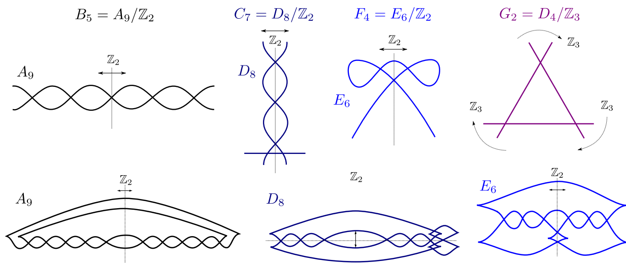
FIGURE 16. Legendrian fronts for \Lambda(A_{2n-1}) , \Lambda(D_{n+1}) , \Lambda(E_6) , \Lambda(D_4) with G -symmetries, G = \mathbb{Z}_2, \mathbb{Z}_3 . The upper row exhibits these symmetric fronts as divides of the associated singularities, and the lower row depicts them in the standard front projection (x, y, z) \mapsto (x, z) for a Darboux chart (\mathbb{R}^3, \xi_{st}) .
