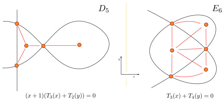
FIGURE 4. The two divides associated to the real morsifications that yield the Lagrangian skeleta in Figures 1 and 2. The implicit equations for the divides are written in terms of the Chebyshev polynomials T_n(w) , determined by the relations T_n(\cos(t)) = \cos(nt) . The (unoriented) quivers associated to these two divides are depicted with orange vertices and red edges. Note that the diagram obtained for E_6 is not the E_6 Dynkin diagram; once the quiver is properly oriented, it is mutation equivalent to an orientation of the E_6 Dynkin diagram.
