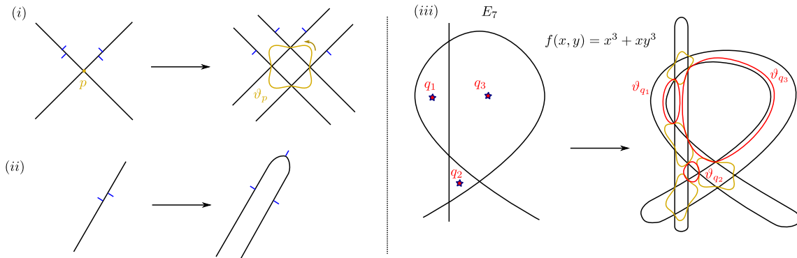
FIGURE 12. (Left) Two front homotopies from the pieces of a divide to a (generic) Legendrian front, in line with the local models in Figure 9. The vanishing cycle \vartheta_p is drawn in the Lagrangian base \mathbb{R}^2 . (Right) A perturbation of a divide for the E_7 -singularity. The vanishing cycles \vartheta_p coming from the double points of the divide are drawn in yellow, and the vanishing cycles \vartheta_q coming from each of the three bounded interior regions are drawn in red.
