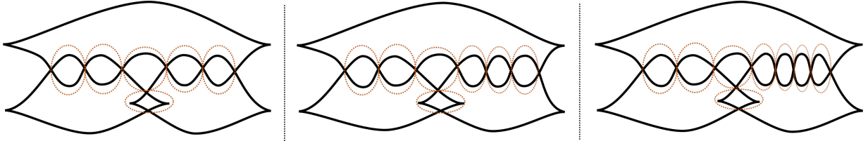
FIGURE 7. The Legendrian links for the E_6, E_7 and E_8 simple singularities.
