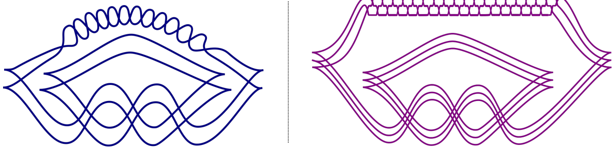
FIGURE 8. The Legendrian links \Lambda_g and \Lambda_h associated to the singularity g(x, y) = x^7 - x^6 + 4x^5y + 2x^3y^2 - y^4 , on the left, and the singularity h(x, y) = x^9 - x^{10} + 6x^8y - 3x^6y^2 + 2x^5y^3 + 3x^3y^4 - y^6 , on the right.
