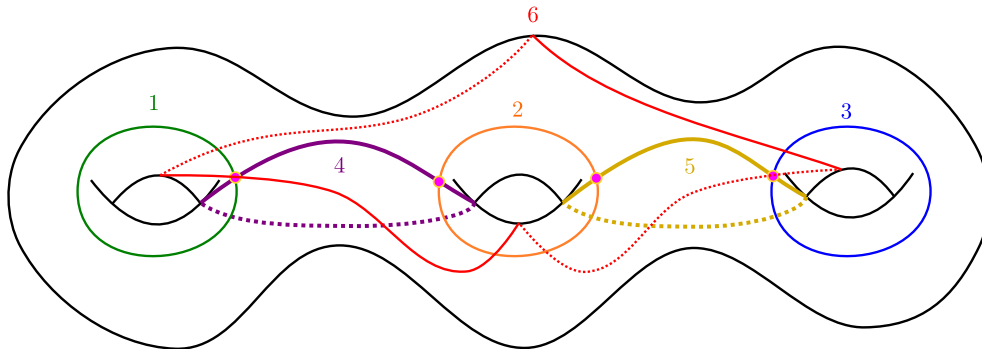
FIGURE 3. Another closed Lagrangian arboreal skeleton for the simple E_6 -singularity f(x, y) = x^3 + y^4 . This is a more symmetric alternative to the closed Lagrangian skeleton in Figure 2.
