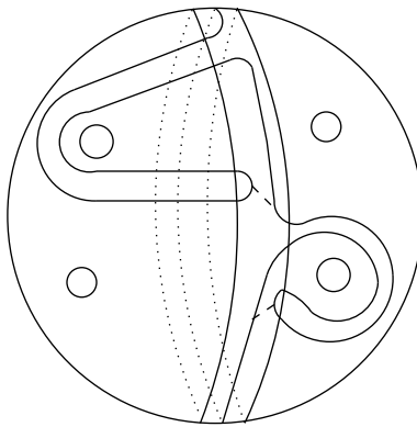
Figure 8: Figure 7 after isotopy
