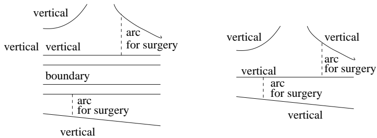
Figure 28: Local picture of amalgamation of pseudovertical Heegaard splittings
