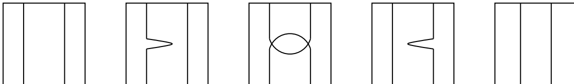
Figure 19: Adding a 1-handle
