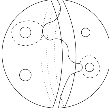
Figure 7: Schematic for vertical Heegaard splittings of graph manifold with boundary
