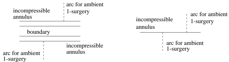
Figure 30: Local picture of amalgamation of Heegaard splittings
