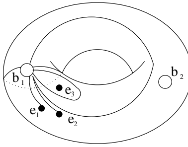
Figure 3: Schematic for a vertical Heegaard splitting of a Seifert fibered space
