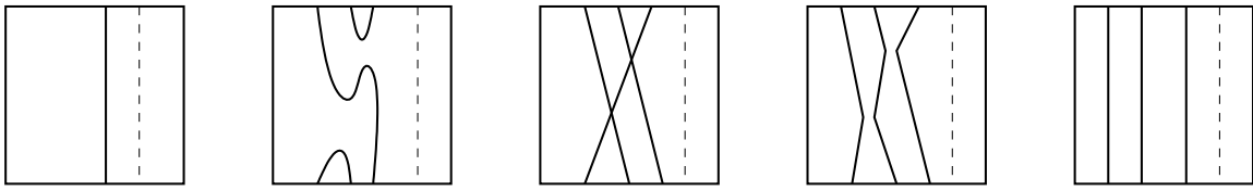
Figure 24: Adding an “essential” 1-handle
