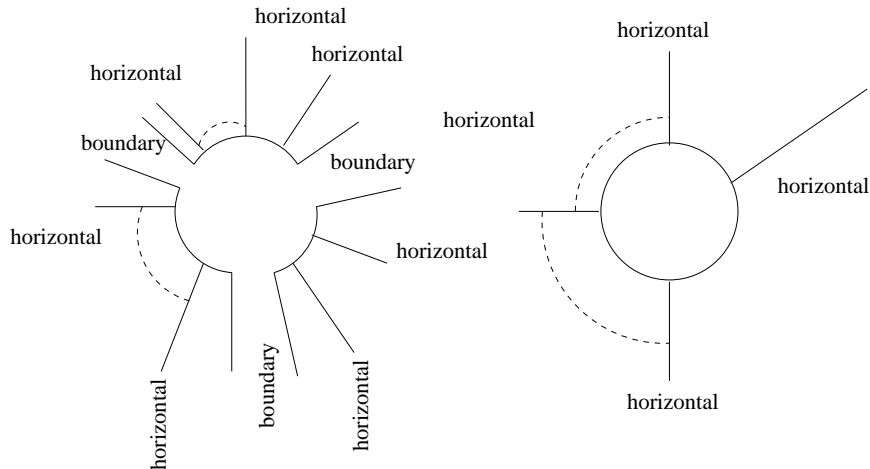
Figure 31: Local picture of amalgamation of Heegaard splittings
