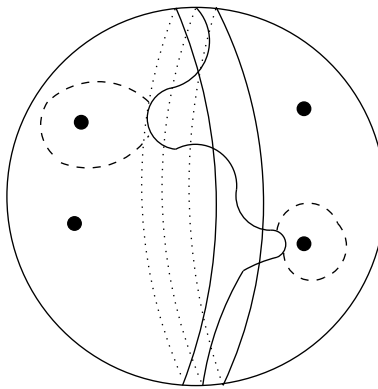
Figure 5: Schematic for Heegaard splitting of a graph manifold
