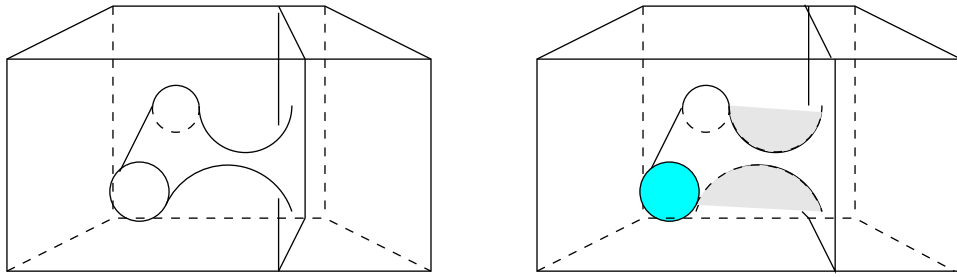
Figure 21: Another stabilized possibility
