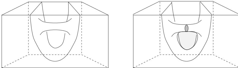
Figure 20: Compressible component meets annulus parallel into T_{t_0 \pm \epsilon}
