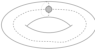
Figure 2: Schematic for Heegaard splitting of Q \times \mathbb{S}^1
