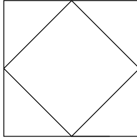
Figure 25: \tilde{G} contains a square
