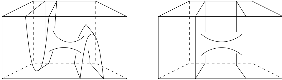
Figure 11: Two isotopic possibilities
