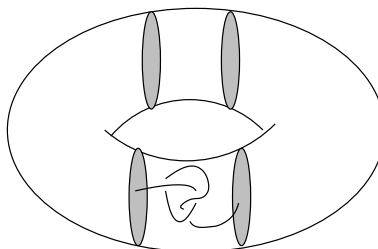
Figure 10: Schematic for a Heegaard splitting intersecting a solid torus
