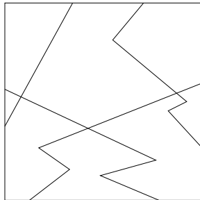
Figure 12: The Rubinstein-Scharlemann graphic
