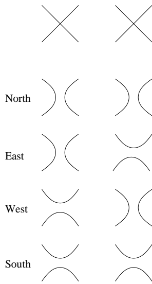
Figure 13: How S_s meets T_t in the four regions North, East, West and South meeting (s_0, t_0)
