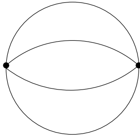
Figure 14: \tilde{G} is contractible
