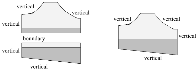
Figure 27: Local picture of amalgamation of vertical Heegaard splittings
