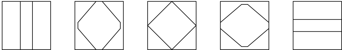
Figure 26: Another way of adding a 1-handle
