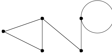
Figure 1: A model graph for a graph manifold
