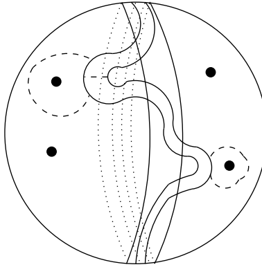
Figure 33: Isotoping the amalgamation into place
