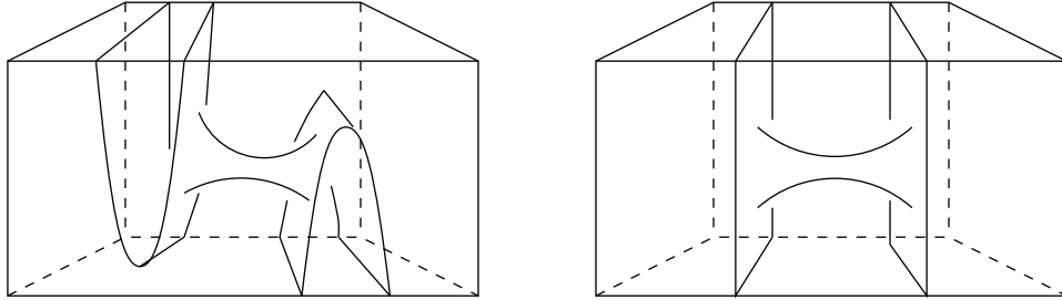
Figure 22: Two isotopic possibilities
