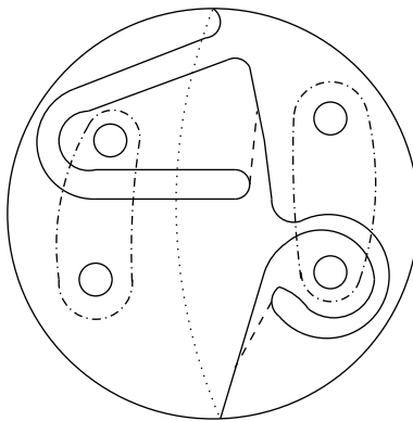
Figure 9: Irregularly dashed arcs indicate new decomposing tori
