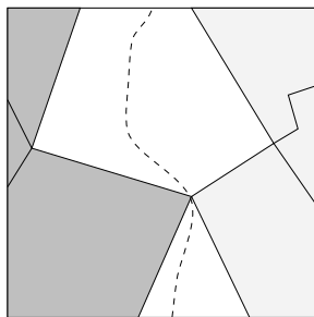
Figure 17: A monotone path through unlabelled regions
