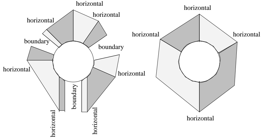
Figure 29: Local picture of amalgamation of horizontal Heegaard splittings
