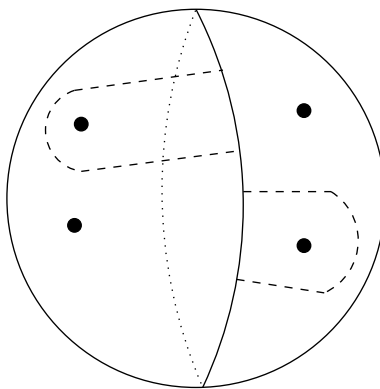
Figure 4: Schematic for Heegaard splitting after amalgamation
