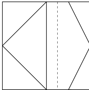
Figure 23: \tilde{G} contains a triangle (dashed arc included along with \tilde{G} to indicate that a bicoloring, as required, is possible)
