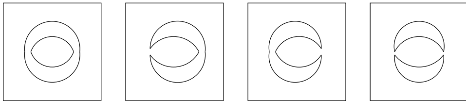
Figure 15: The regions North, East, West and South
