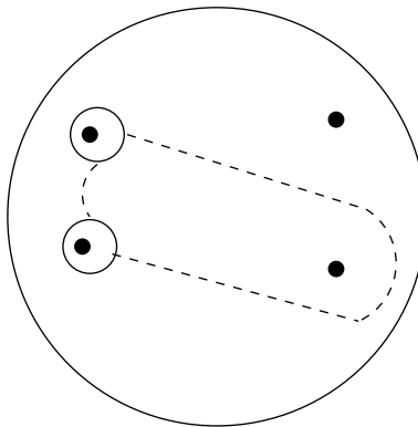
Figure 6: Schematic for Heegaard splitting of a Seifert fibered space
