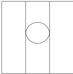
Figure 18: \tilde{G} contains a bigon
