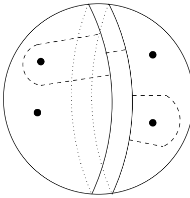
Figure 32: Amalgamating to obtain an edge manifold
