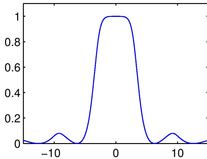
\Phi(\xi), m=1
