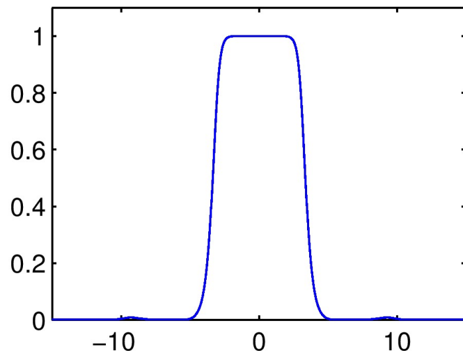
\Phi(\xi), m=3
