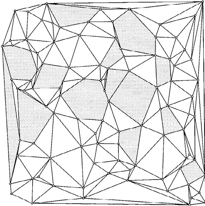
Fig. 3. The light edges for a set of 100 points. The faces which are not triangles are shaded.
