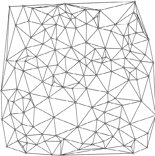
Fig. 4. Minimum weight (light) triangulation for 150 points.
