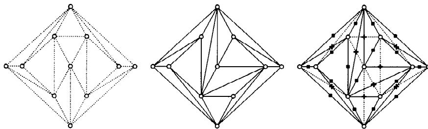
Fig. 1. Two triangulations and a perfect matching between them. When two identical edges are matched this is indicated by a small box, and the intersection point of two crossing edges which are matched is marked by a cross.
