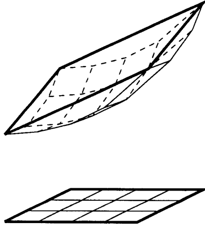
FIGURE 3. \mathcal{P}_2(4, 3) and \tilde{\mathcal{P}}_3(4, 3)
