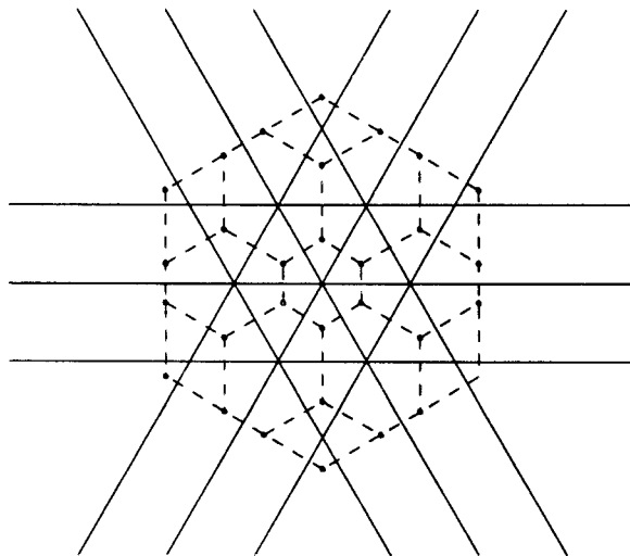
FIGURE 4. The polar complex
