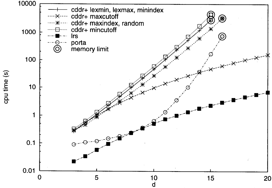
Figure 4: CPU time for dwarfed cubes, rational arithmetic
