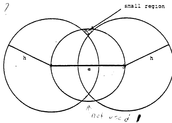
Figure 2: When e has length less than \sqrt{3}h , the triangle's vertex must lie within this small region.
