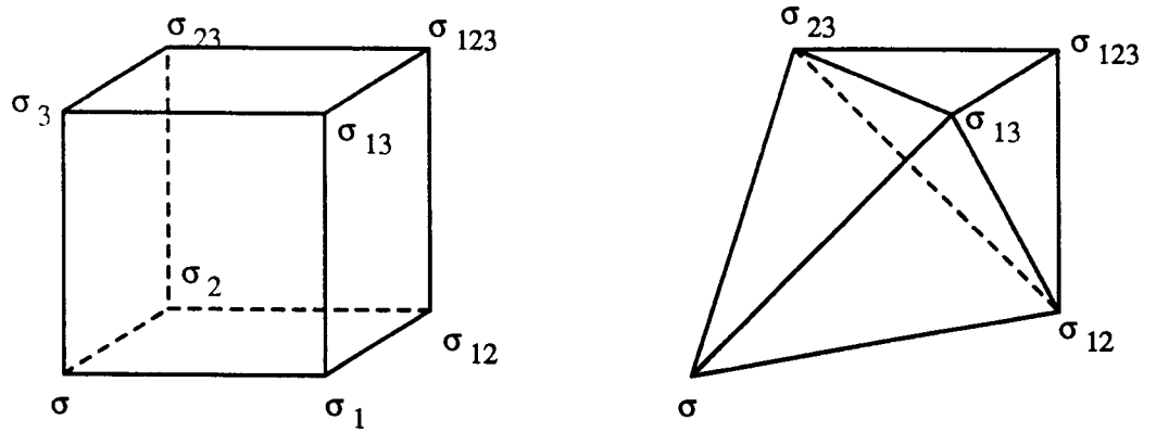
Figure 1: F(\sigma, \mathcal{C}) and F'(\sigma, \mathcal{C}) for Example 1
