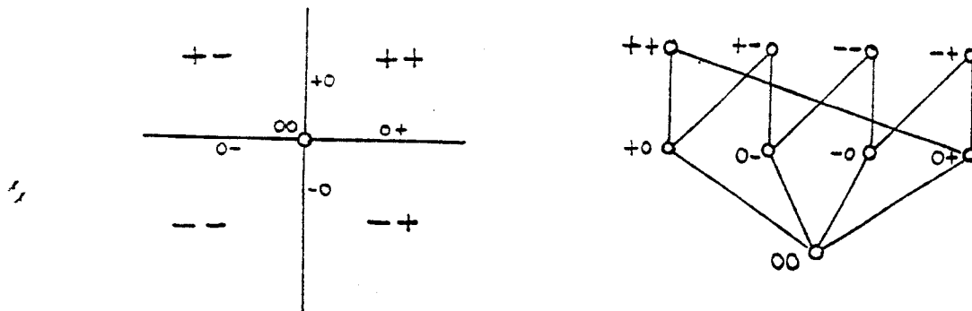
Figure 2.2: s^{(2)} , and its poset of signs.
