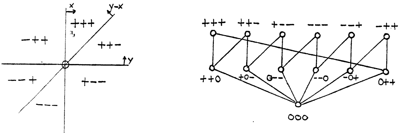
Figure 5.1. Face poset \mathcal{L} of an arrangement of three lines in \mathbb{R}^2 .
