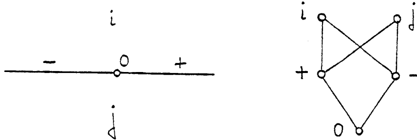
Figure 2.1: s^{(1)} , and its poset of signs.
