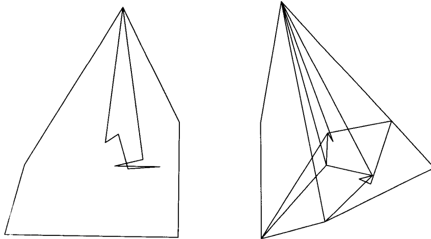
Figure 9. The fold curves for two projections of the tight polyhedral projective plane with a handle; each can be broken into fold curves in more than one way. The projection onto the xy plane (left) can be broken into one or two components depending on the decision made at the topmost vertex, h . The other projection (right) can be broken into as many as six components; it has three interior vertices where more than two fold edges meet. There are projections for which the fold curves are even more complicated.
