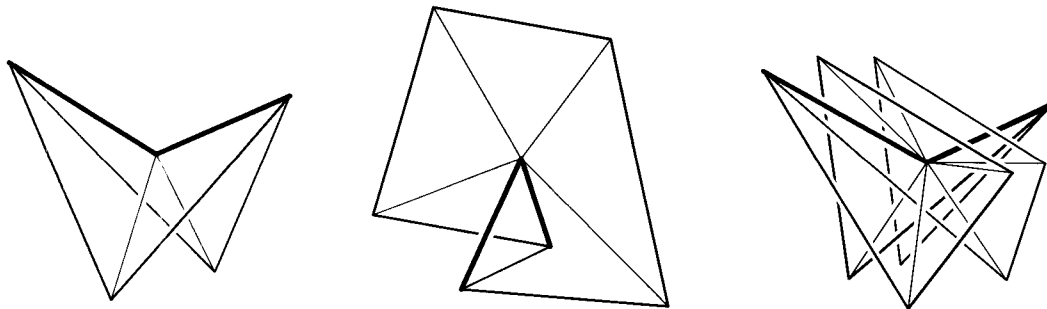
Figure 10. Polyhedral analogues of the fold and cusp (left). The neighborhood of a vertex can wrap around the vertex an arbitrary number of times (right), though only a single revolution is shown here. The fold edges themselves do not contain enough information to distinguish between the two folds shown.
