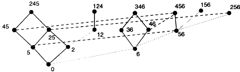
Figure 3. M -shelling of the lower-bound poset for Example 3
