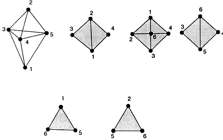
Figure 2. PS ear-decomposition of the matroid complex of Example 3
