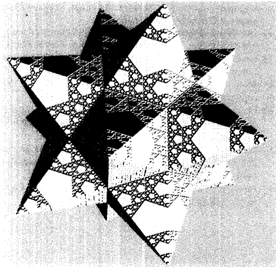
Fig. 8. Dodecafoam filling the stellated dodecahedron.
