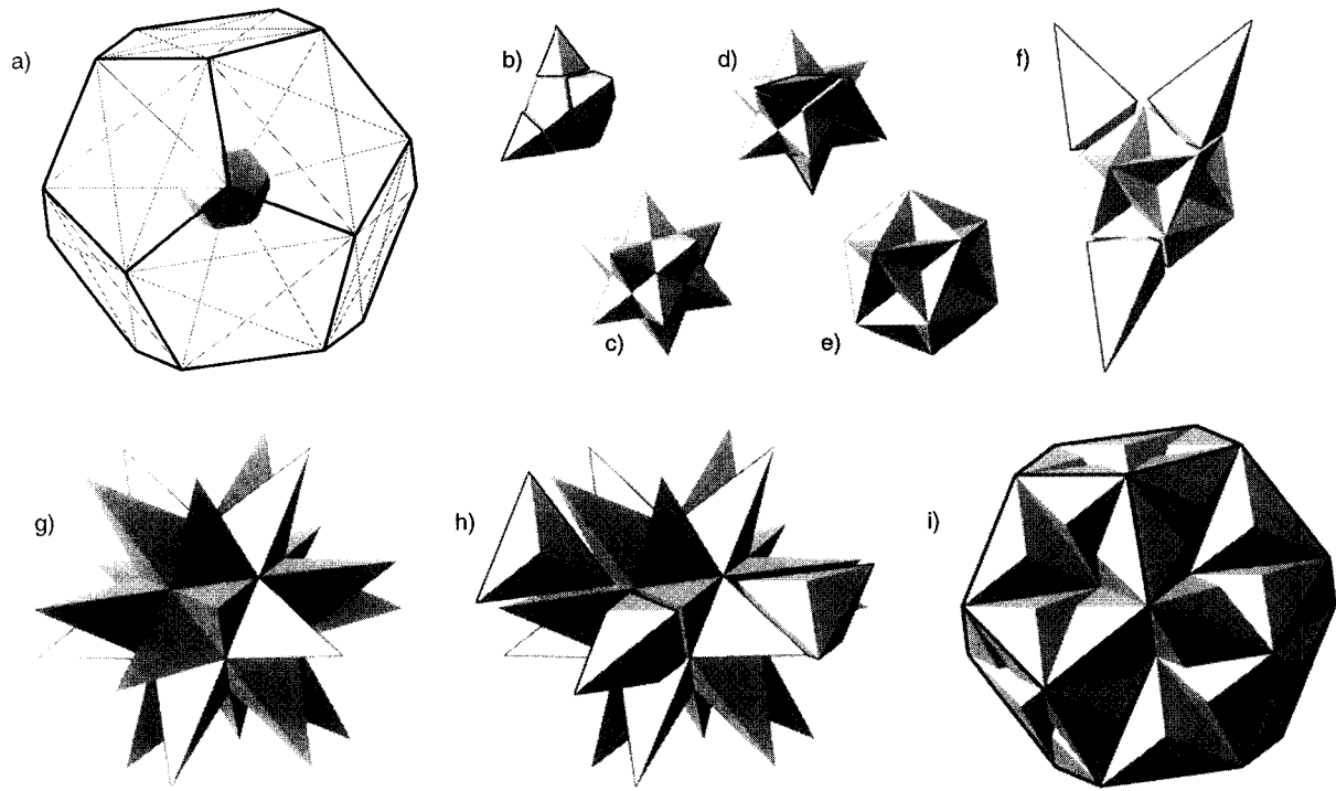
Fig. 5. Examining the faceted D_3 .
