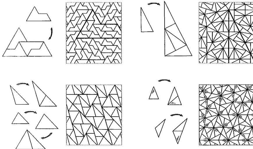
Fig. 2. Several substitution tilings.
