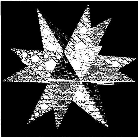
Fig. 11. Dodecafoam filling the great stellated dodecahedron.
