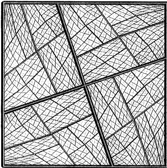
Fig. 3. A projective substitution tiling.
