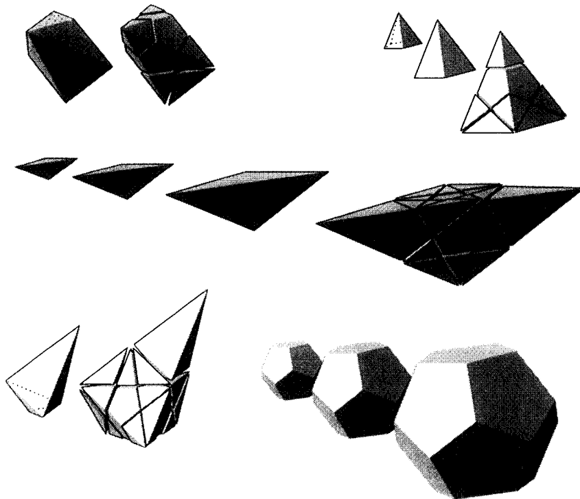
Fig. 6. Substitutions.
