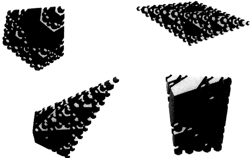
Fig. 7. Filling the cells with dodecahedra.
