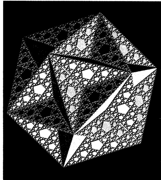
Fig. 10. Dodecafoam filling the great dodecahedron.
