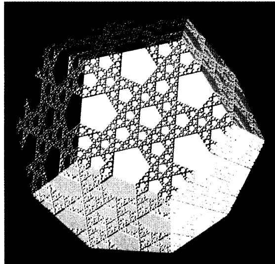
Fig. 9. Dodecafoam filling a dodecahedron.
