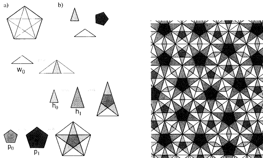
Fig. 1. A pentagonal substitution tiling.
