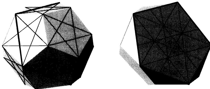
Fig. 4. Faceting D_3 .
