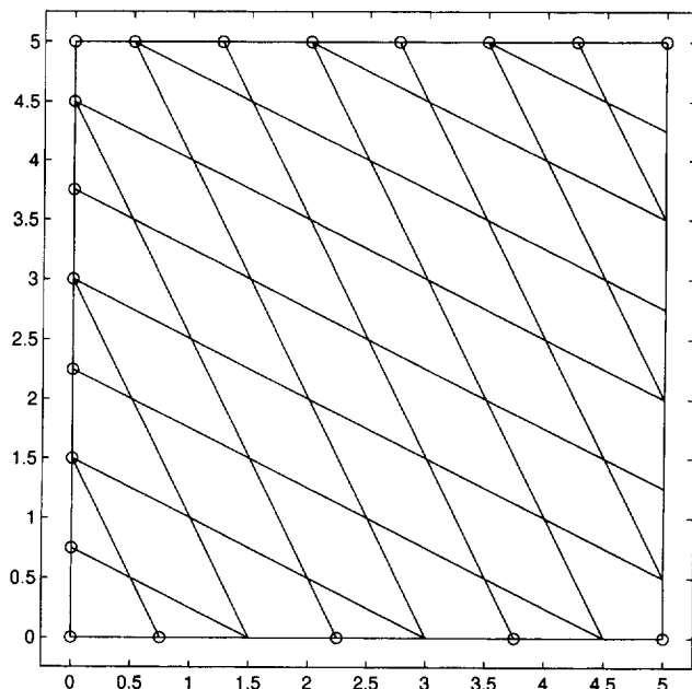
Fig. 3. Remaining candidate points (depicted by o) after applying Lemma 6.1.
