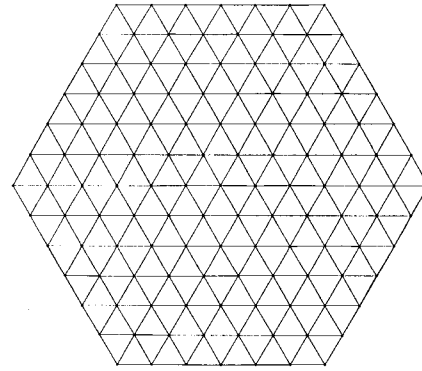
Fig. 6. Case of triangular grid: Application of Nemhauser and Trotter's 'skeletal' approach
