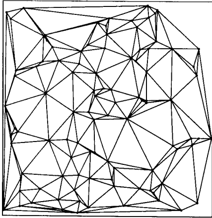
Fig. 1. Minimum weight triangulation of a set of 100 points
