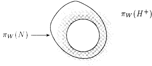
Figure 2. \pi_W(N) rings the hole of \pi_W(H^+) .
