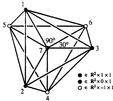
Fig. 2. \psi|_{\mathbf{N}} as seen from above.
