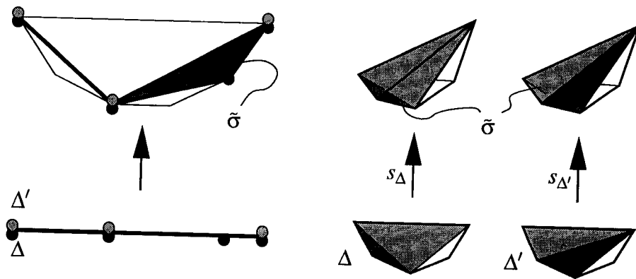
Figure 2. Increasing flips in \mathcal{S}_1(6, 1) respectively \mathcal{S}_1(5, 2) .
