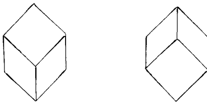
Fig. 4. The two coherent tilings of a (1, 1, 1) hexagon.
