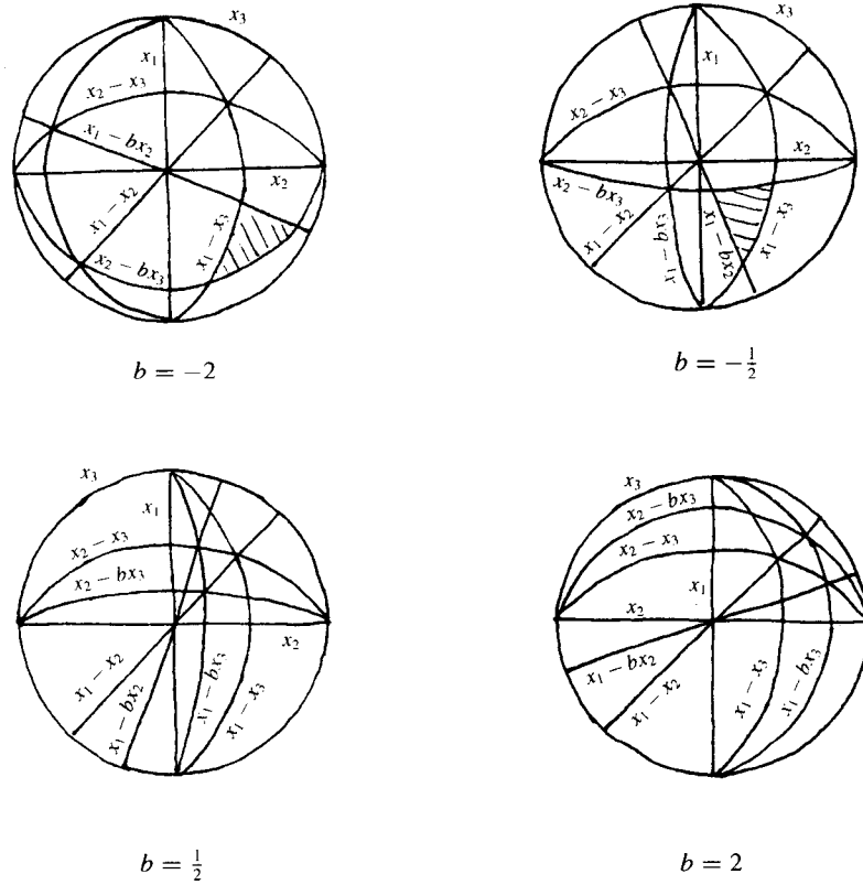
Fig. 10. \mathcal{A}_{=,1,1,1}^{(b)} for b = -2, -\frac{1}{2}, \frac{1}{2} , and 2 .
