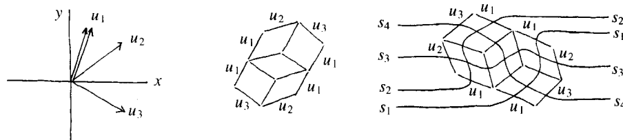
Fig. 11. A tiling and its braid picture.
