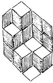
Fig. 1. Picture of a plane partition as a bunch of stacked cubes.
