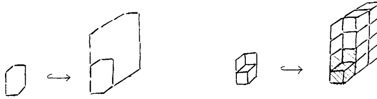
Fig. 8. Extending a tiling of Z to one of Z' .
