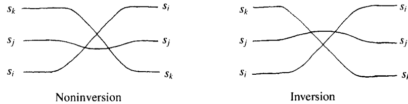
Fig. 12. The two orders in which three strands can cross.
