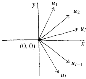
Fig. 7. The convention for ordering the zonotope generators.
