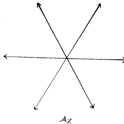
Fig. 6. The discriminantal arrangement \mathcal{A}_{Z(1,2,1)} .
