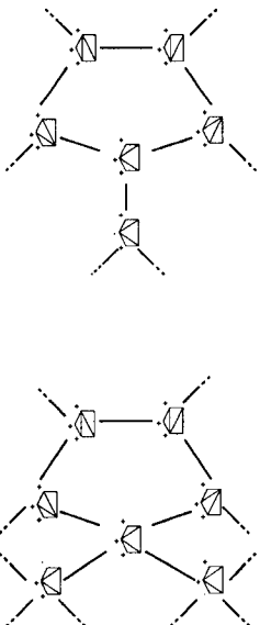
FIGURE 2. A part of the graph for (a) the simple signed associahedron, (b) the non-simple signed associahedron
