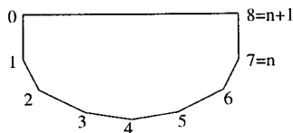
FIGURE 1. The labelling of vertices in the (n + 2) -gon \mathcal{P}_n .
