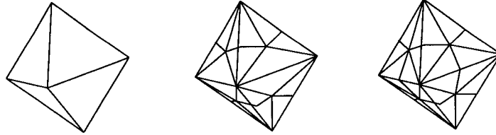
FIGURE 5. \Delta_0, \Delta^* \simeq (\mathbb{K}_n^B)^* and \Sigma_n^B when n = 3
