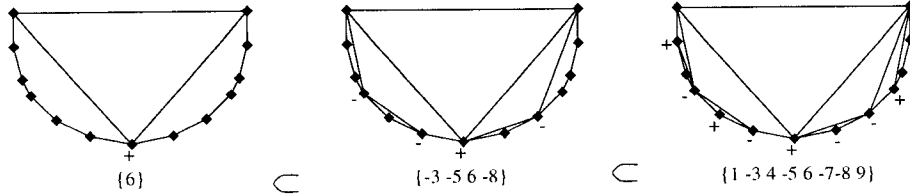
FIGURE 6. The map \psi : A chain of isotropic subsets S_1 \subset S_2 \subset S_3 of \{\pm 1, \pm 2, \dots, \pm 11\} , and the associated signed dissection
