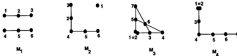
FIGURE 1. Matroids M_1 and M_2 have the same Tutte polynomial and the same spectrum polynomial. Matroids M_3 and M_4 have the same Tutte polynomial but different spectrum polynomials.
