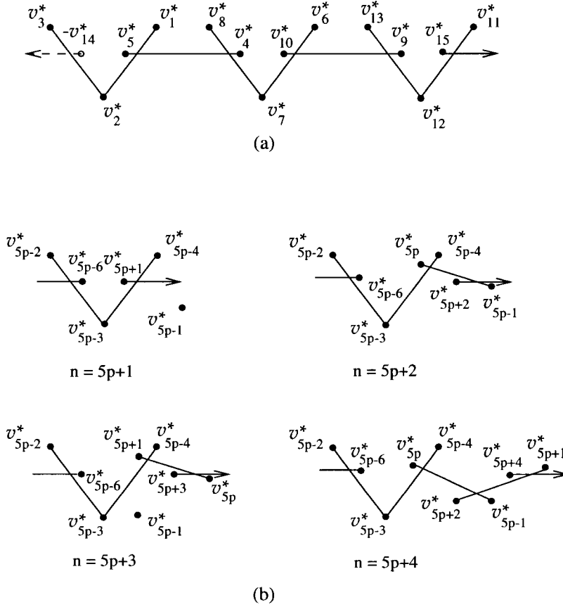
FIGURE 2. Few flips in corank 3.
