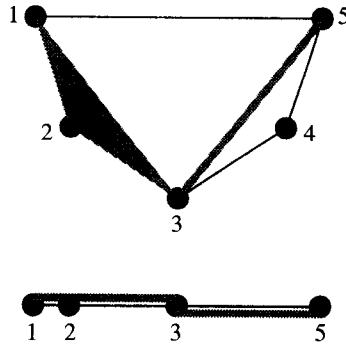
FIGURE 1. The subdivision \{123, 35\} of C(5, 1) , induced by the cells 123 and 35 of the subdivision \{123, 135, 345\} of C(5, 2) .
