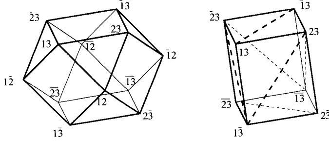
Figure 3: A cuboctahedron (left) and a square prism inscribed in it, with diagonals inserted in its facets (right).
