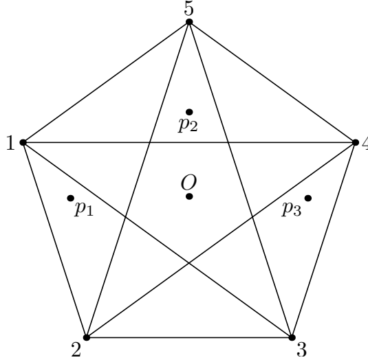
Figure 5: Pebbles and \text{cov}(x) for a pentagon
