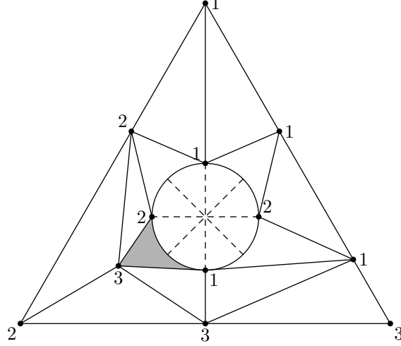
Figure 6: Sperner's lemma for the Möbius band
