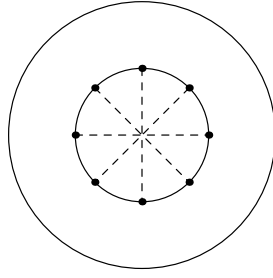
Figure 3: Möbius band. Diametrically opposite points of the inner boundary circle are to be identified. The outer circle is the boundary of the Möbius band.
