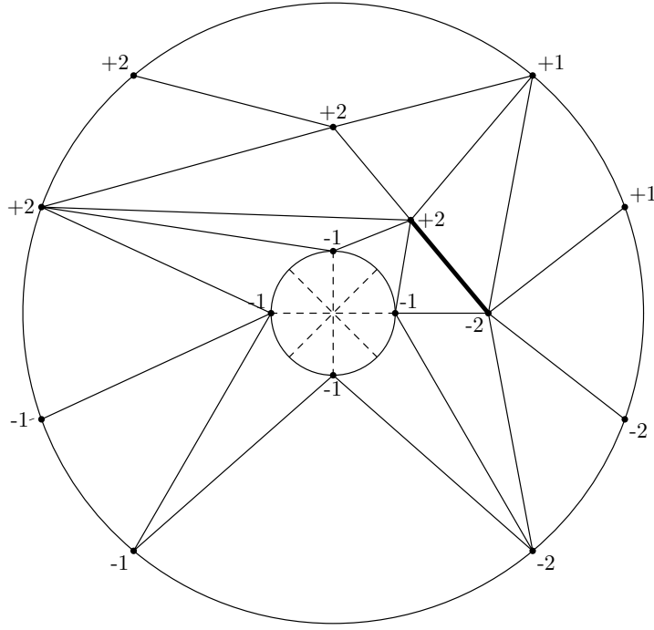
Figure 7: Tucker's lemma for the Möbius band
