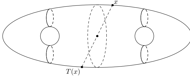
Figure 4: The double torus that is centrally symmetric embedded to \mathbb{R}^3 .
