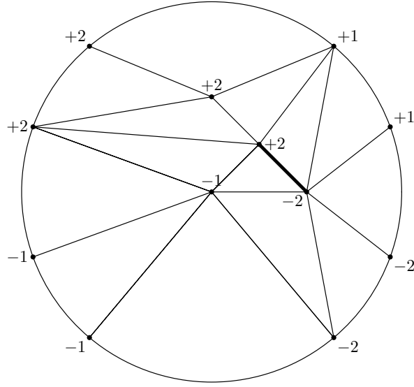
Figure 2: A 2-dimensional illustration of Tucker's lemma
