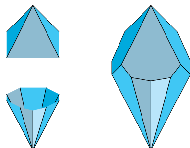
Figure 2. A 3-spindle (picture courtesy of F. Santos)
