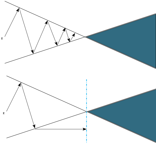
Figure 9. The standard relaxation method projects only on given constraints (top), Chubanov's variation (bottom) allows for the generation of new constraints that speed up convergence.
