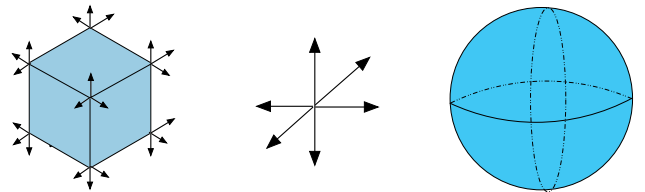
Figure 5. The normal fan of a regular 3-cube has eight cones (left), which coincide with the eight possible orthants (center). To visualize and study the fan, we intersect it with the unit sphere. This yields a decomposition of S^2 into eight spherical triangles (right). The resulting map on the surface of the sphere is a combinatorial octahedron.
