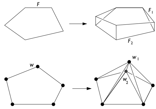
Figure 4. A wedge construction and its dual the one point suspension (courtesy of Edward D. Kim)
