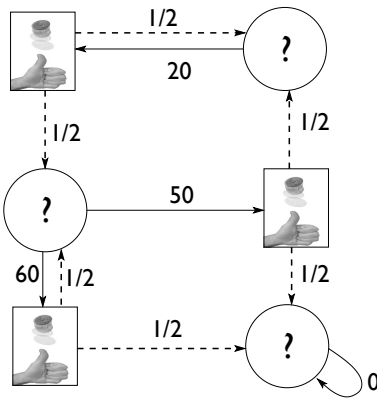
Figure 7. An example of an MDP graph encoding the process
