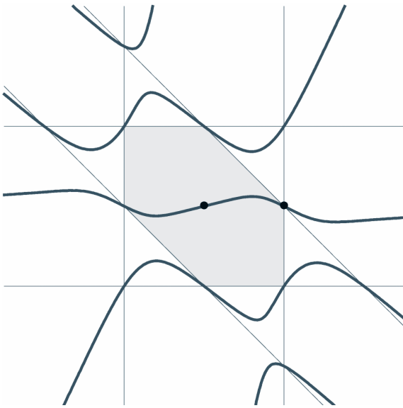
Figure 10. A view of the entire central curve of a linear program
