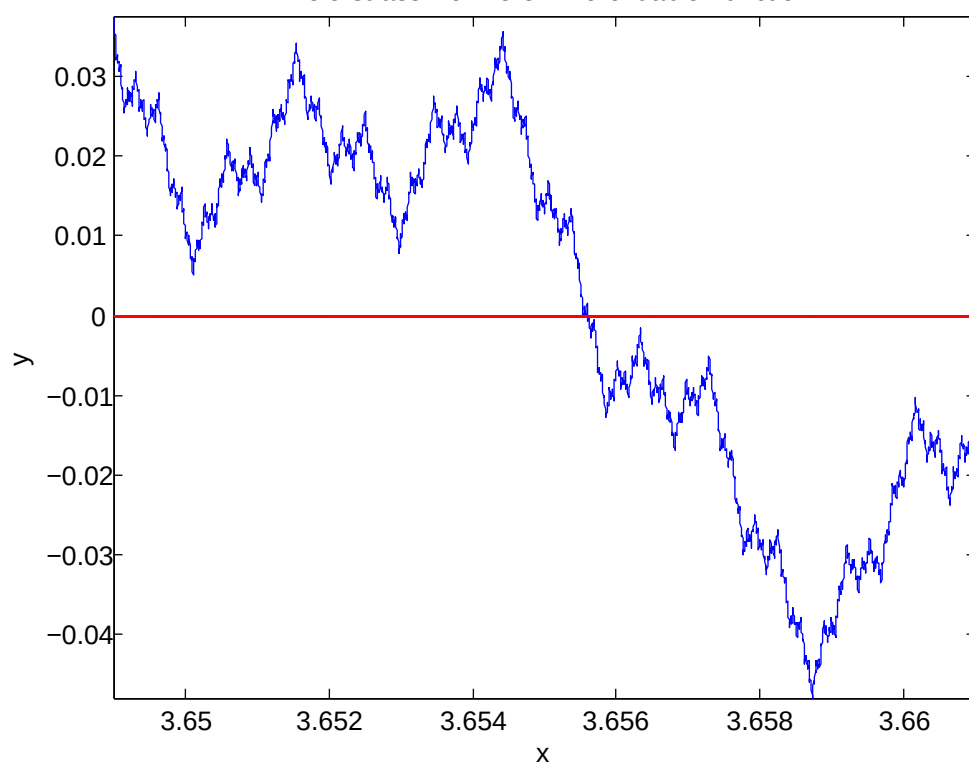
Weierstrass Nowhere Differentiable Function
