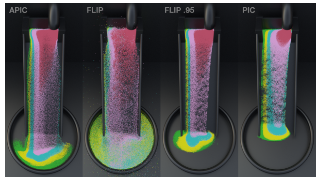
Figure 3: We compare APIC with PIC, FLIP and FLIP/PIC blends for an MPM simulation of granular materials. Notice PIC and FLIP/PIC blend are stable but exhibit overly viscous behavior, while pure FLIP is unstable and noisy as evidenced by stray particles and excessive mixing. APIC however is both stable and nearly dissipation free. ©Disney.
