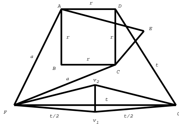
Fig. 13. The based Peaucellier straight-line motion linkage \tilde{\mathcal{S}} : \ell[v_1v_2]^2 + (t/2)^2 = \ell[Fv_2]^2 = \ell[Gv_2]^2 . The image of B under all realizations lies on a segment of the real axis which contains the open interval (-\sqrt{3}/2)t, (\sqrt{3}/2)t \subset \text{Dom}^*(\tilde{\mathcal{S}}) .
