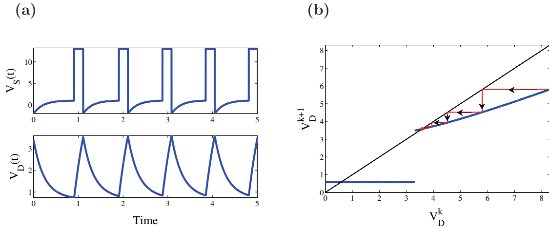
Figure 10. The ping-pong effect and bistability in the two-compartment model with the square spike. (a) Voltage traces of the somatic and dendritic compartments with the square spike as in (7.1). For the parameter values used, I < I_{th} = 2.6 , and the ping-pong effect between the somatic and dendritic compartment potentials holds the system in the oscillatory regime. (b) The grey line plots the return map (6.4) derived from the two-compartment model with the square spike. The black line is identity line V_D^{k+1} = V_D^k . The map has two stable fixed points indicating that the full two-compartment model displays bistability between periodic firing and the quiescent steady state: The lower fixed point corresponds the quiescent steady state (V_D^{ss}, V_S^{ss}) , and the upper fixed point corresponds to periodic firing. Parameters for both plots are \beta = 13 , T_a = 0.2 , V_R = -2 , g = 1.5 , g_{lk} = 2 , \alpha = 1 , and I = 2.5 .
