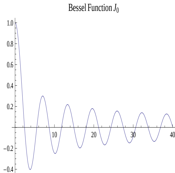
Figure 6.5: The Bessel function J_0(x) . First zero occurs at approximately 2.4048, the second zero at 5.5201, the third zero at 8.6537, \dots
